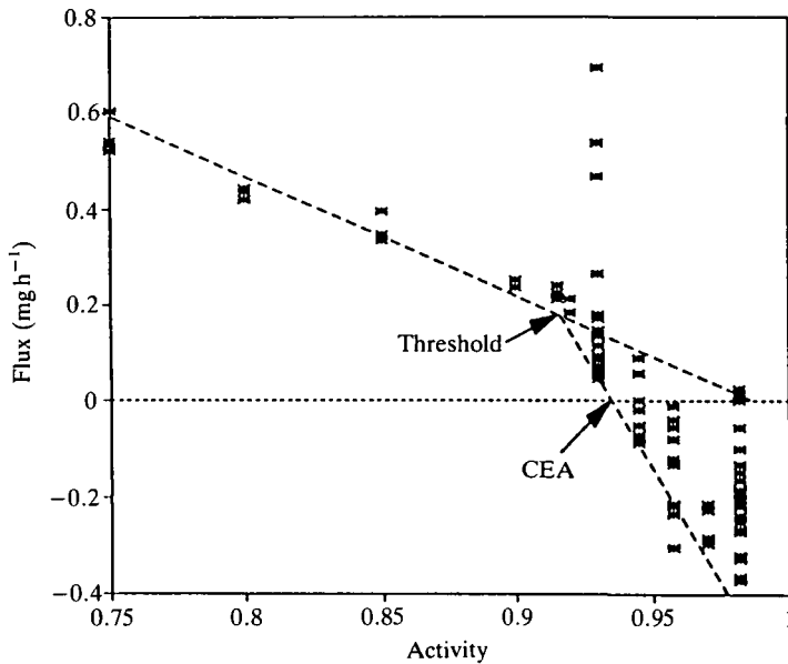
Fig. 2. Example plot of variation in net flux with external water activity for Armadillidium vulgare . Positive fluxes (passive losses) vary as a direct function of external activity, indicating near-stable, gradient-independent permeability. Haemolymph and external vapour are in dynamic equilibrium (stable mass) at an activity of about 0.99. Below the regression line for passive losses, flux may be reduced (above the threshold) or reversed (above the CEA) by WVA. Uptake rates are variable in a given external activity, but maximum rates suggest a linear increase in WVA with relative humidity; the uptake mechanism thus shows non-saturated kinetics.
