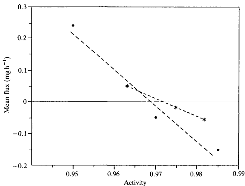
Fig. 6. Plots of uptake flux ( \text{mg h}^{-1} ) against external water activity for two specimens of Porcellio scaber employing sustained WVA during continuous gravimetric monitoring. Increased uptake fluxes were accompanied by concurrent increases in pleopodal ventilation frequency (see Table 4). The observed linear relationships suggest uptake fluid of constant osmolality, but differing in each case. The CEA estimates (at zero uptake flux) show that neither animal is employing WVA at the maximum rate. Lines are fitted by eye.
